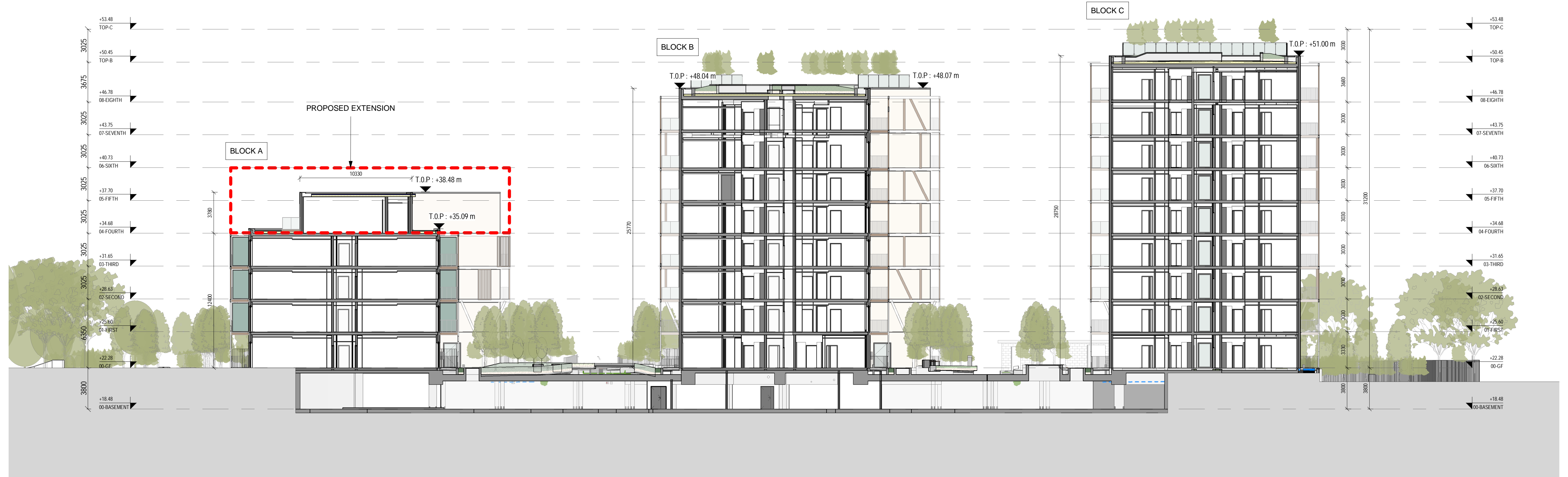
① LONGITUDINAL SECTION - THROUGH BLOCKS - A, B & C - PROPOSED Scale: 1 : 200
