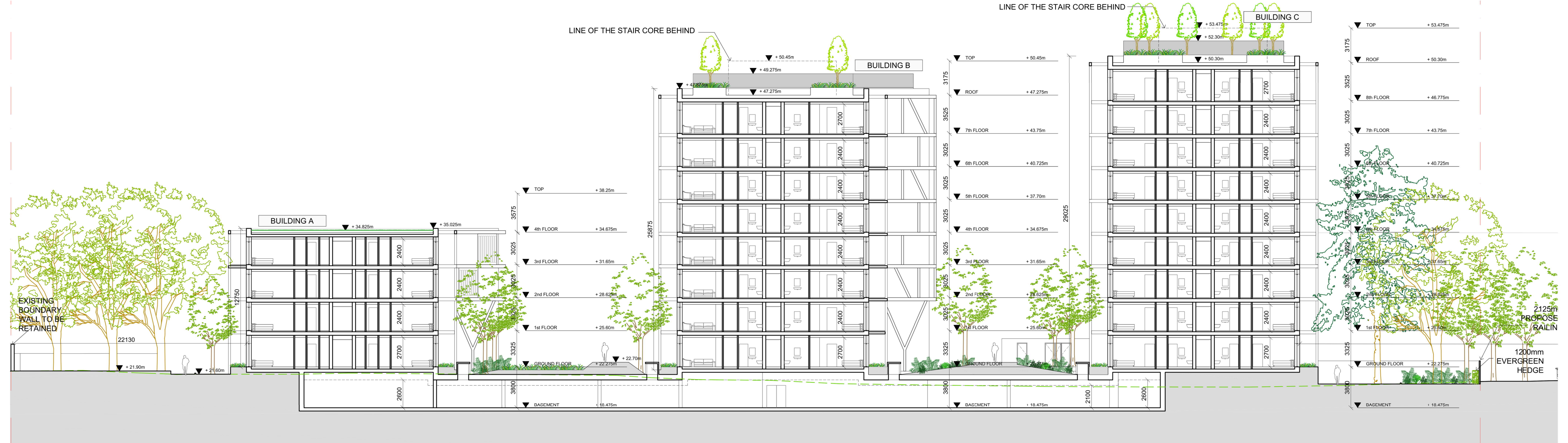
② LONGITUDINAL SECTION - THROUGH BLOCKS - A, B & C - EXISTING PLANNING Scale: 1 : 200
