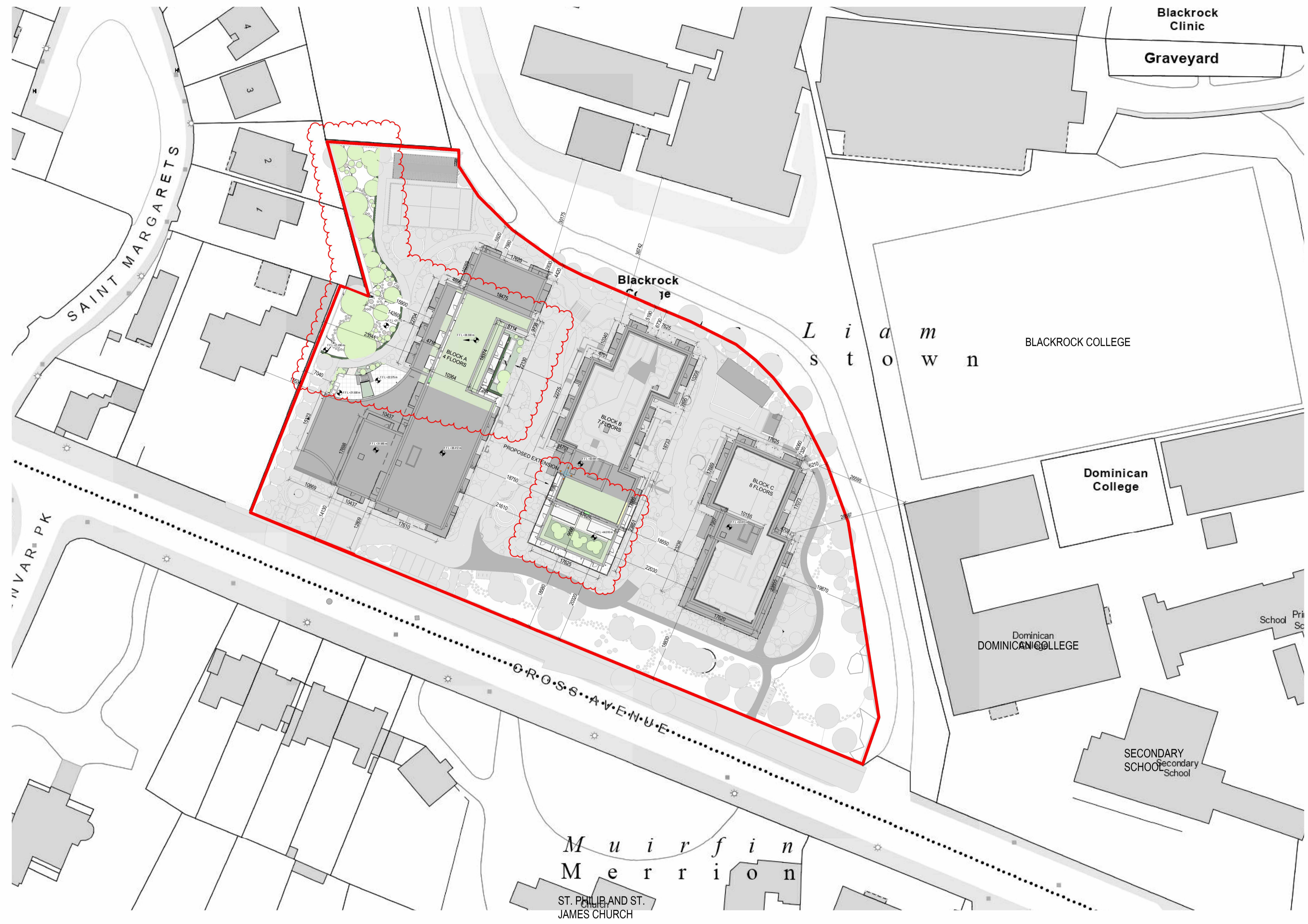
2 PLANNING PROPOSED SITE PLAN Scale: 1 : 500
